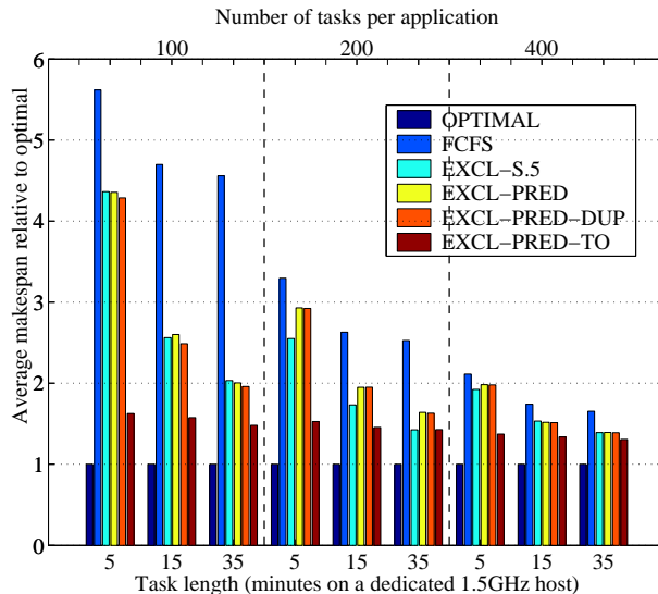
Figure 10: Heuristic performance using replication on SDSC grid
